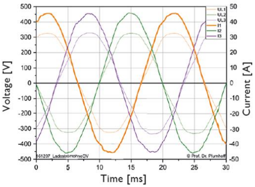
FIGURE 2: CHARGING CURRENT WITHOUT LIMIT VIOLATION
