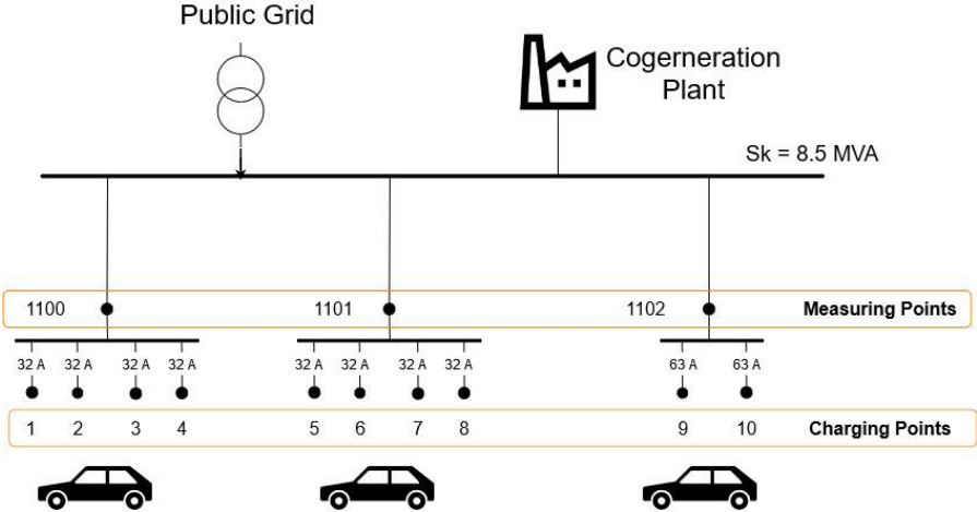
FIGURE 1: CIRCUIT DIAGRAM OF THE CHARGING STATION
